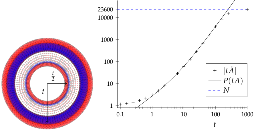
FIGURE 7. Annuli: comparison of the penguin valuation P(tA) = 3t^2/8 + 3\pi t/4 with |t\check{A}| , an approximation to the magnitude.
